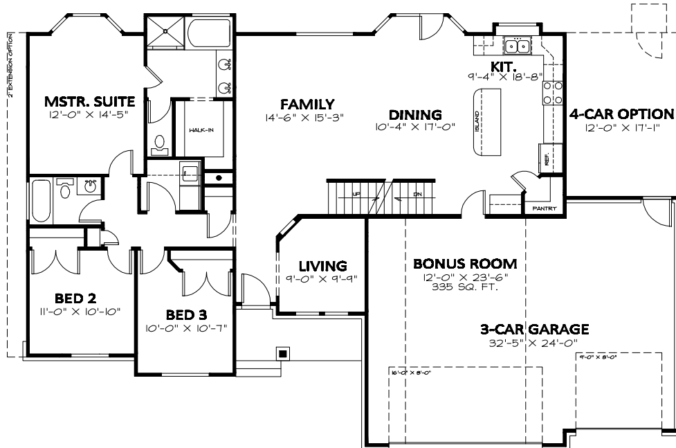
Main Level
