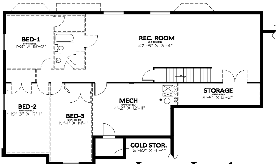
Lower Level
