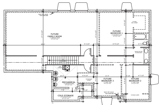
Lower Level: 1864 Sq. Ft.
